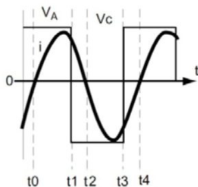
Figure 11. Waveform of the Main Power Circuit
