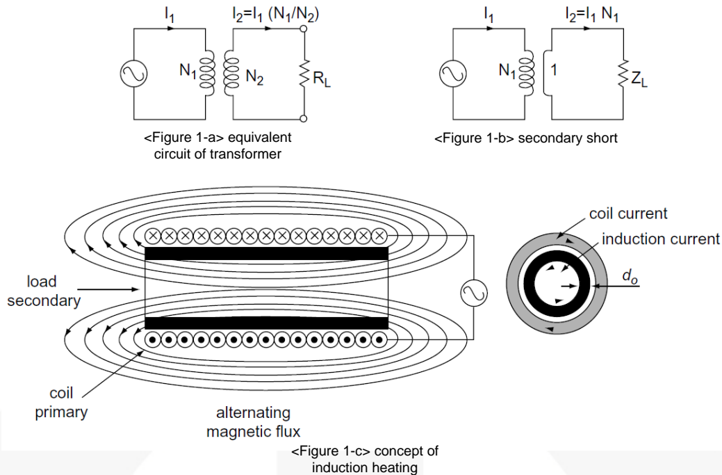
Figure 1. Basics of Induction
